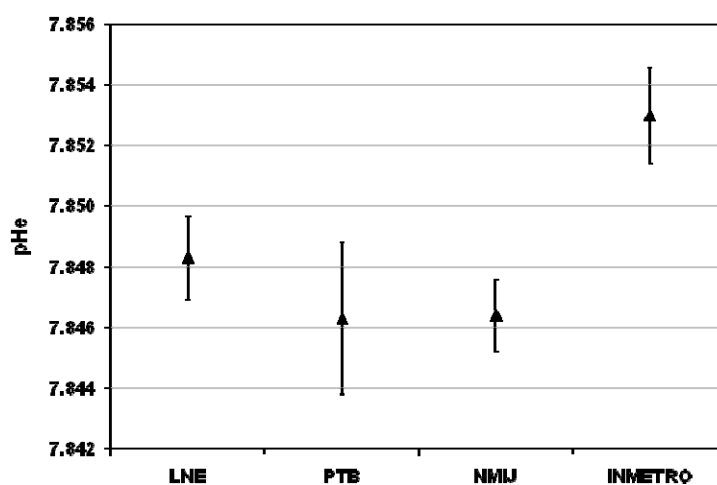
Figure 3. Comparison of pH measurement using the Harned cell system amongst four national measurement institutes of 0.03 mol/kg phosphates in 50 % EtOH-H 2 O mixture. vertical bars correspond to the uncertainty (k=1) of the acidity function (intercept to zero chloride molality)
